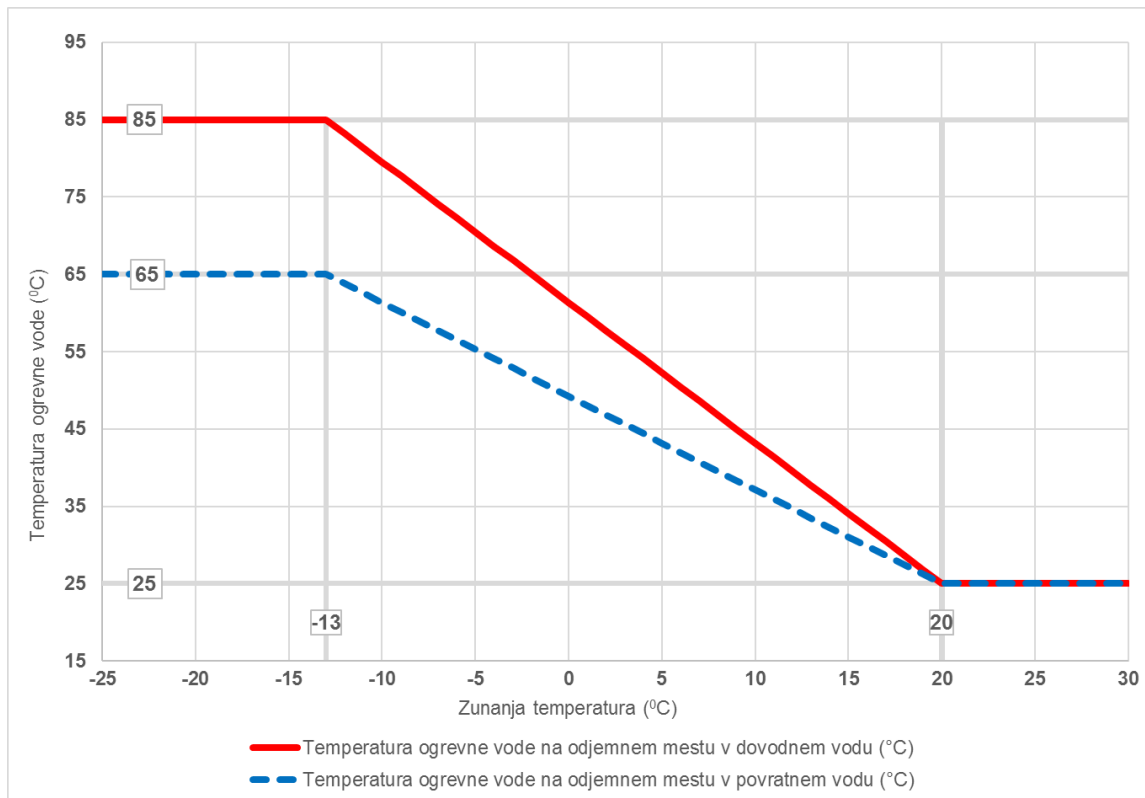
Diagram 6: Temperaturni diagram za zunanjo normno temperaturo -13^{\circ}\text{C} (interni razvod 85/65^{\circ}\text{C} , NP 3)
